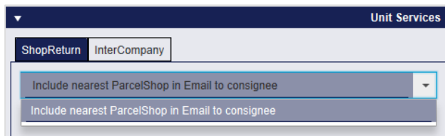
Figure 154 – ShopReturnService
