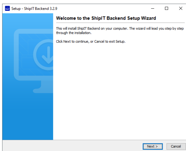
Figure 3 – Installer: Welcome
