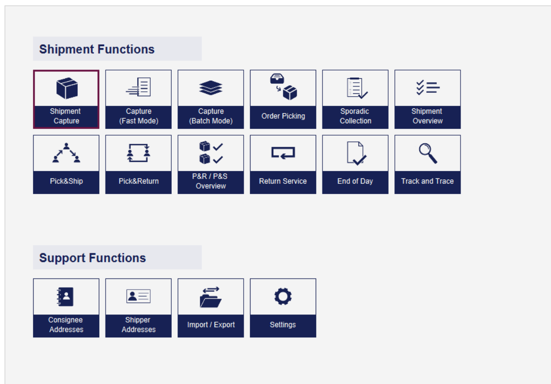
Figure 38 – Main menu
