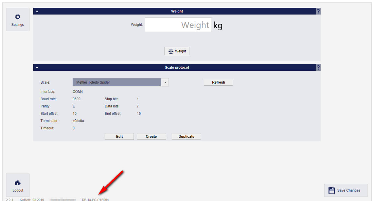
Figure 79 – Scale Settings
