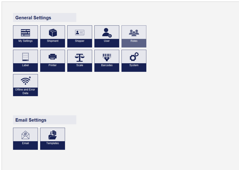
Figure 51 – Settings
