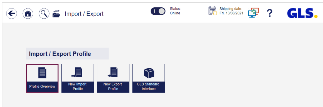
Figure 161 – Import / Export
