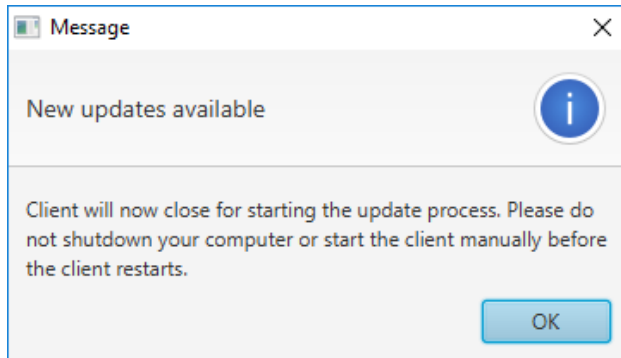
Figure 26 – Updates available
