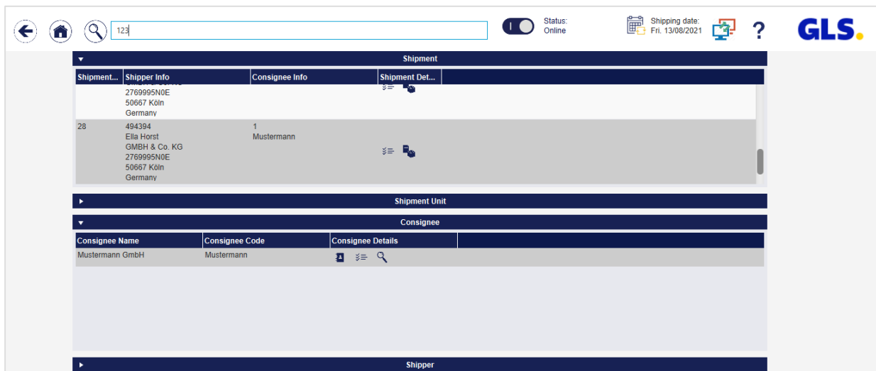
Figure 35 – Search
